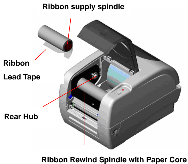
Fig. 5 Ribbon installation (II)
