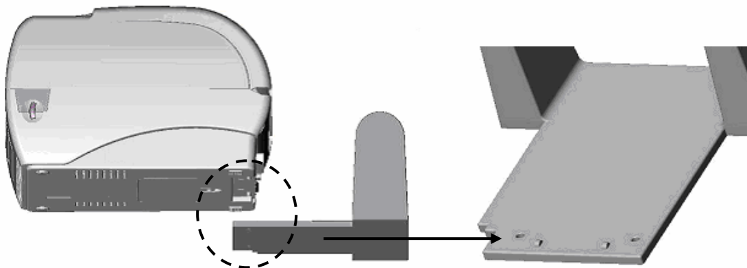
Fig. 9 Attach the external roll mount to the printer
