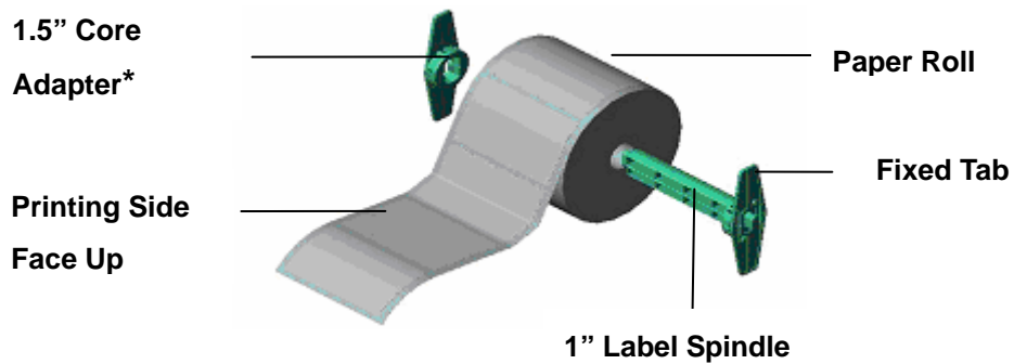
Fig. 6 Label roll installation (I)
