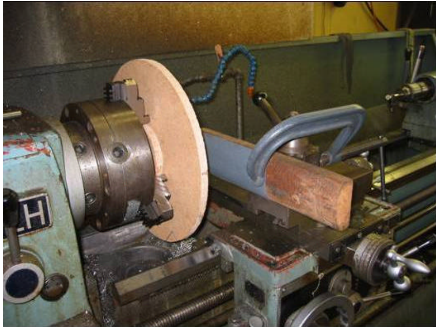
Figure 7. Abrasion Station (Back View)
